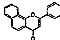
α-NAPHTHOFLAVONE
